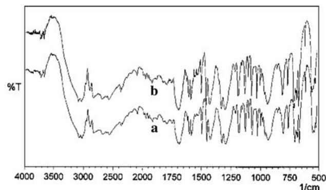
Fig. 7 Diffuse reflectance FTIR (DRIFT) spectra of trans -stilbene, (a) standard and (b) isolated product (mp = 122 °C)
