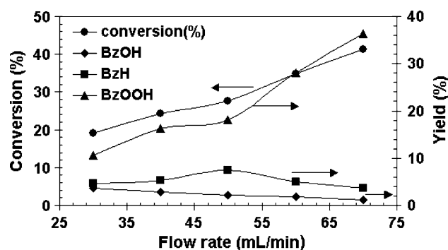
Fig. 5 Effect of flow rate of oxygen on the oxidation of toluene. Reaction conditions: catalyst (0.4 g), toluene (20 mL), pO_2 (101 kPa), temperature (90 °C), stirring (900 rpm), time (3 h)
