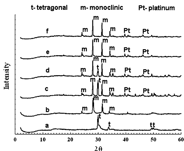
Fig. 2 XRD pattern of ZrO 2 and Pt/ZrO 2 . (a) ZrO 2 (uncalcined), (b) ZrO 2 (calcined at 950 °C), (c) Pt/ZrO 2 (unreduced, calcined at 750 °C) and (d) Pt/ZrO 2 (calcined at 750 °C and reduced in H 2 ). (e) Pt/ZrO 2 (unreduced, calcined at 950 °C) and (f) Pt/ZrO 2 (calcined at 950 °C and reduced in H 2 )
