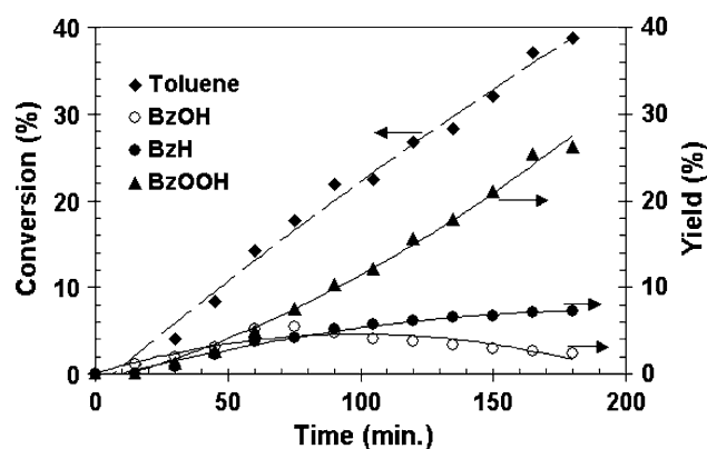
Fig. 3 Time profile for the oxidation of toluene. Reaction conditions: catalyst (0.2 g), toluene (10 mL), pO 2 (101 kPa), flow rate (40 mL/min), temperature (90 °C), stirring (900 rpm)
