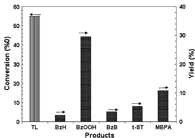
Fig. 6 Conversion of toluene after 7 h of reaction. TL: toluene, BzH: benzaldehyde, BzOOH: benzoic acid, BzB: benzyl benzoate, t -ST: trans -stilbene, MBPA: methyl biphenyl carboxylic acid reaction. Conditions: toluene (20 mL), catalyst (400 mg), pO_2 (101 kPa), flow rate (40 mL/min), agitation (900 rpm), temperature (90 °C)
