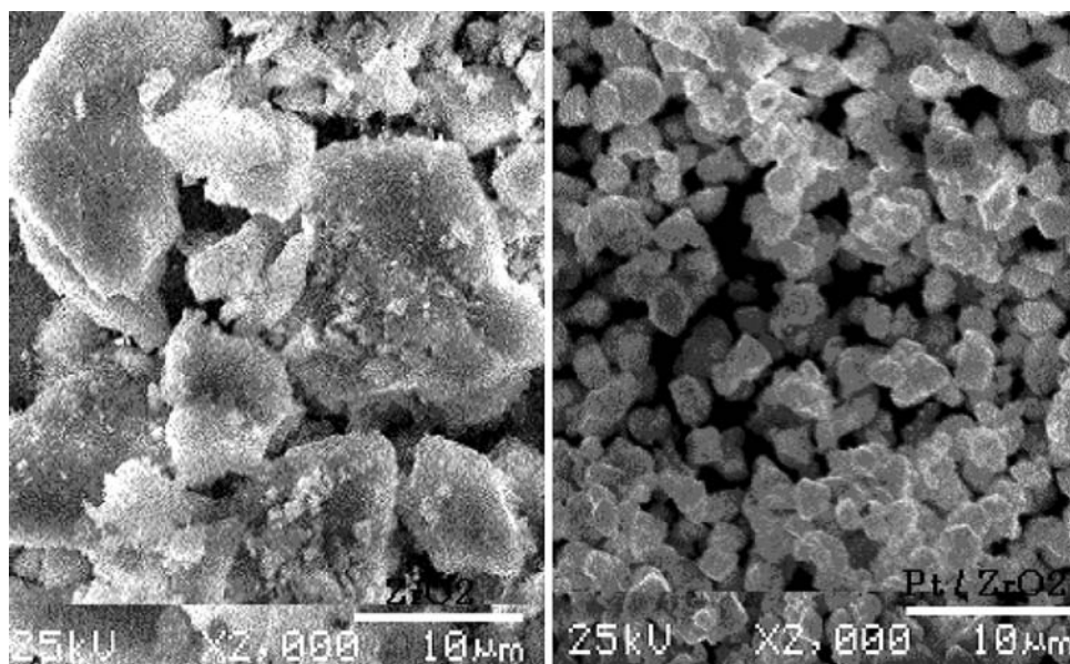
Fig. 1 SEM images of ZrO 2 (calcined at 950 °C) and Pt/ZrO 2 (calcined at 950 °C and reduced in H 2 )
