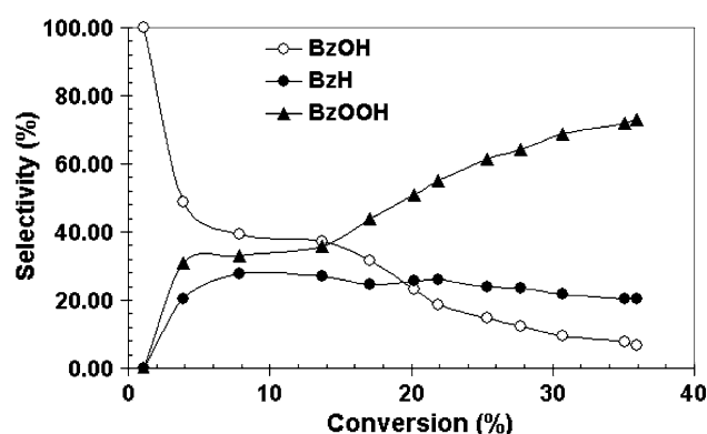
Fig. 4 Selectivity of toluene oxidation at various conversions. Reaction conditions: catalyst (0.2 g), toluene (10 mL), pO 2 (101 kPa), flow rate (40 mL/min), temperature (90 °C), stirring (900 rpm)
